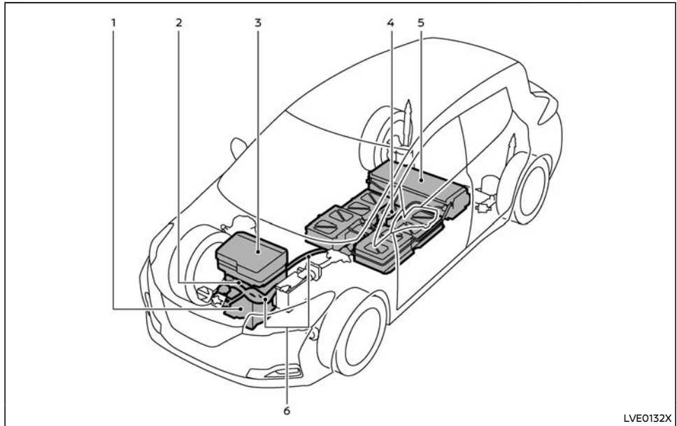
High-voltage components
