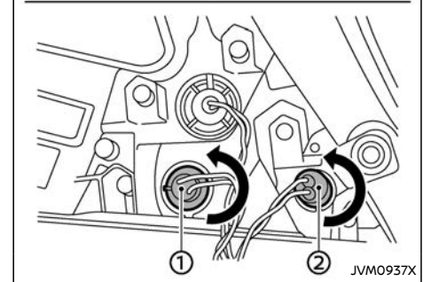
Rear combination light
